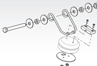
PosiLift™ Guide Arm and Bearing Block Part No. 48100498 SRK-632
