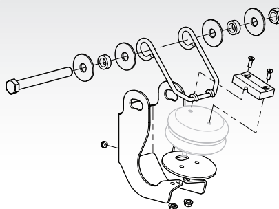
PosiLift™ Bracket Replacement Kit Part No. 48100496 SRK-630
