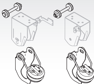
Bolt-On PosiLift™ Kit* Part No. 44100160 SRK-0055
